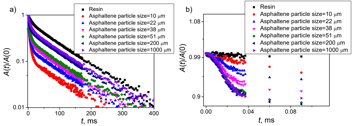
Figure 3. a) Normalized to the amplitude at the initial moment of time ( t = 0 ) relaxation attenuations for the resin and resin samples containing 10 % asphaltenes with different particle sizes (shown in the figure) obtained by using the pulse sequences solid-echo and CPMG; b) The initial areas of relaxation attenuations shown in figure 3a. Measurements were made at a temperature of 310 K.
