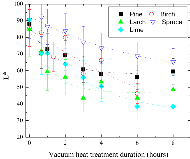
Figure 2. Evolution of L^* parameter values as a function of the vacuum heat treatment duration for spruce, lime, pine, birch and larch samples. The temperature of heat treatment is 220^\circ\text{C} . Dotted lines represent envelope curves.
