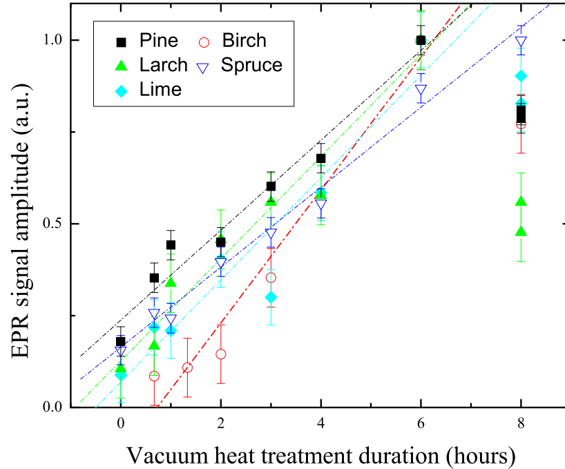
Figure 1. The normalized EPR signal amplitude of birch, lime, larch, spruce and pine samples as a function of the vacuum heat treatment duration at 220°C. Dash-dot line represents the linear behaviour of the obtained data from 0 h to 6 h.
