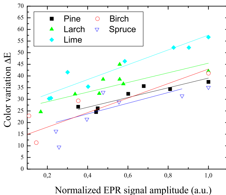
Figure 5. Correlation between the color variation \Delta E and the normalized EPR signal amplitude of heat-treated spruce, lime, pine, birch and larch samples. Solid lines represent the linear correlation. The temperature of heat treatment is 220°C.
