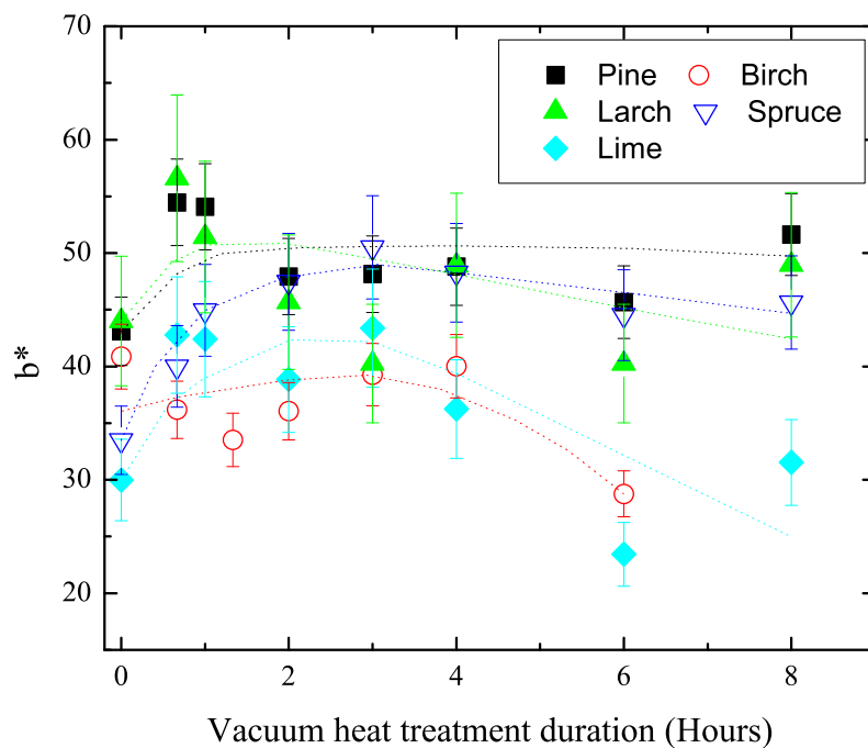
Figure 4. Evolution of b^* parameter values as a function of the vacuum heat treatment duration for spruce, lime, pine, birch and larch samples. The temperature of heat treatment is 220°C. Dotted lines represent envelope curves.
