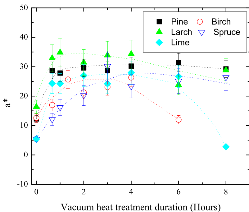
Figure 3. Evolution of a^* parameter values as a function of the vacuum heat treatment duration for spruce, lime, pine, birch and larch samples. The temperature of heat treatment is 220°C. Dotted lines represent envelope curves.
