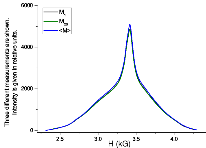
Figure 1. (Color online) Here we demonstrate the EPR resonance line for the chosen sample. All measurements are located inside the limited ones. The mean measurement \langle y \rangle (blue line) serves as envelope. It signifies about the accuracy of the equipment used. Being plotted with respect to the mean curve their corresponding slopes ( \text{slope}(y_2, \langle y \rangle) = 1.04648 , \text{slope}(y_{21}, \langle y \rangle) = 1.05429 ) are very close to the unit value.
