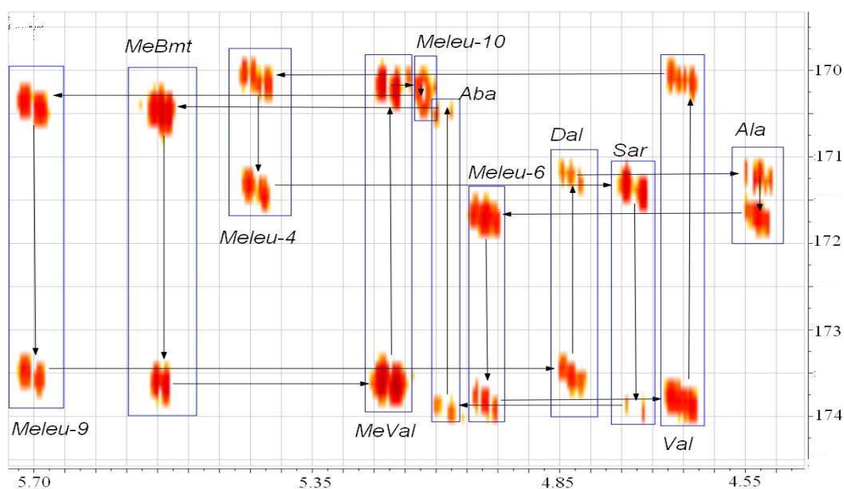
Figure 2. HMBC ( ^1\text{H} 500.13 MHz, ^{13}\text{C} 125.76 MHz) spectrum of cyclosporine in chloroform at T = 293 K. Region of correlations between \text{C} = \text{O} and \text{NCH}_3 groups is shown.
