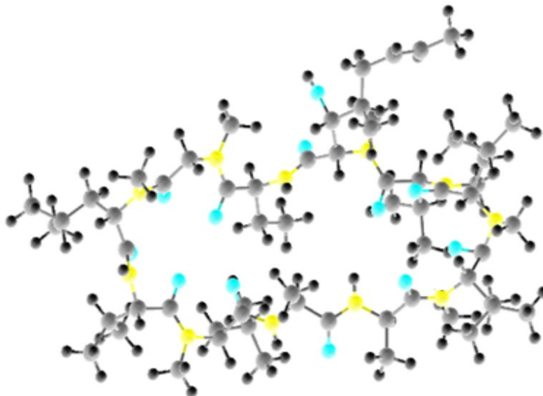
Figure 3. Averaged spatial structure of cyclosporine in chloroform after final energy minimization.
