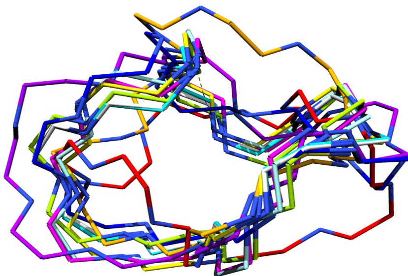
Figure 4. Backbones of 10 lowest energy structures.
