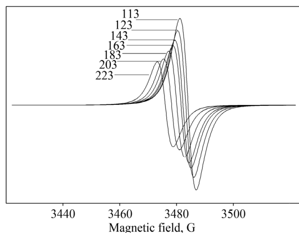
Figure 5. Temperature dependency (K) EPR spectra of the nanocomposite of silver and VT-AN copolymer.
