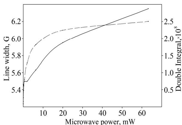
Figure 4. Dependency of signal width (solid line) and double integral (broken line) on microwave power for colloidal silver nanoparticles containing VT-AN nanocomposite.
