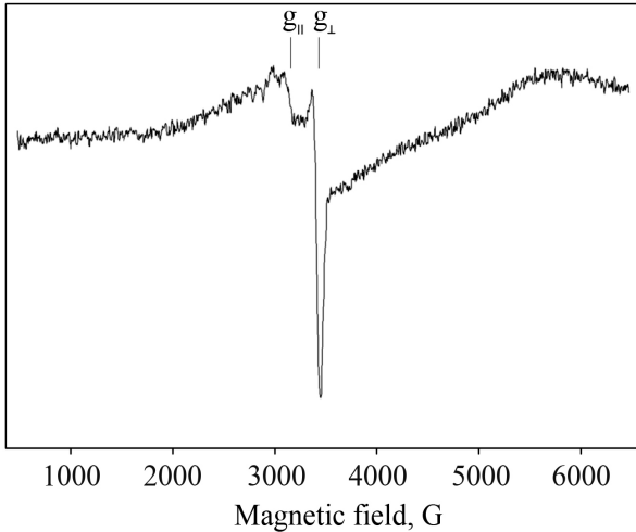
Figure 1. EPR spectrum measured at room temperature for the polymeric complex of the VT-AN copolymer with \text{AgNO}_3 , where g_{||} = 2.2623(2) , g_{\perp} = 2.0762(2) .
