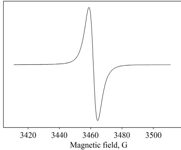
Figure 2. EPR spectrum measured at room temperature for colloidal silver nanoparticles containing VT-AN nanocomposite.
