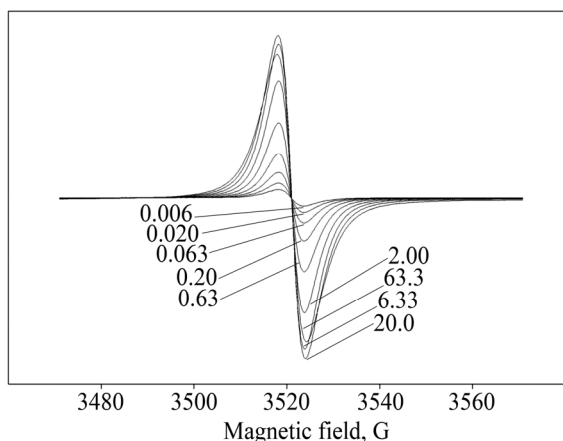
Figure 3. EPR spectra measured at room temperature for the nanocomposite of silver and VT-AN copolymer at various microwave powers (mW).
