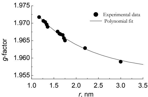
Figure 2. g -factor of the shallow donor as a function of ZnO nanoparticles size. The fitting function is g(r) = 1.98835 - 0.01724 \cdot r + 0.00248 \cdot r^2 , where r is in nanometers.
