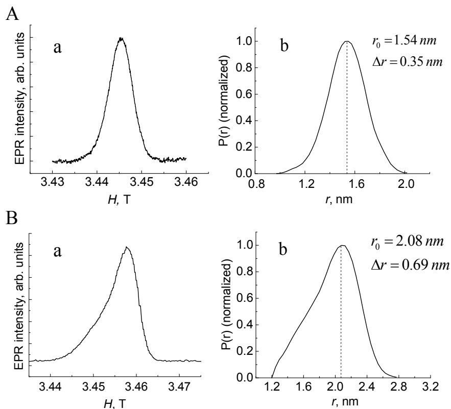
Figure 3. EPR spectrum (a) and estimated size distribution function (b) of two samples (A and B) of ZnO nanoparticles. r_0 is the size, corresponding to the peak of the distribution, \Delta r_0 is the distribution width on the half-height.
