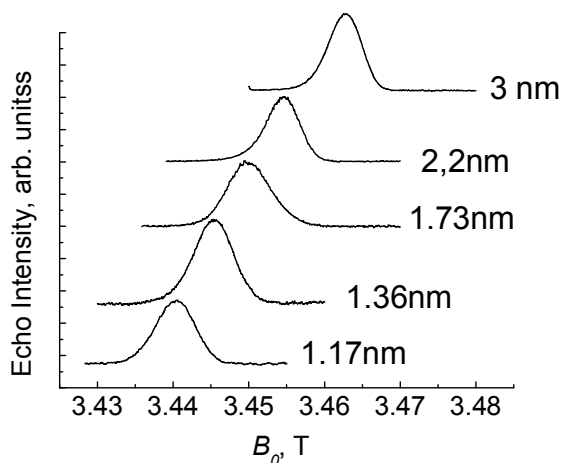
Figure 1. Position of the shallow donor EPR line in ZnO nanocrystals is strongly correlated with the size of the nanocrystals, f = 94.9 GHz.
